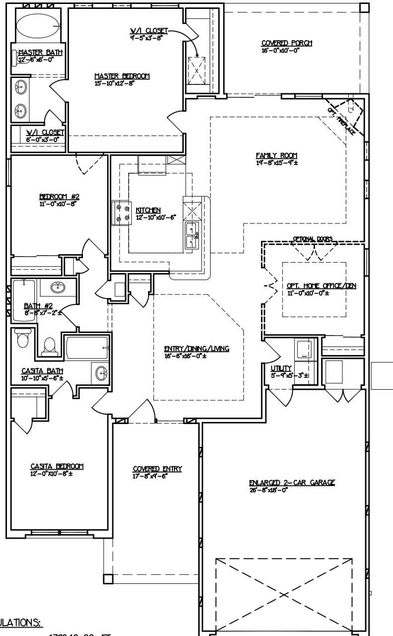
FLOOR PLAN
