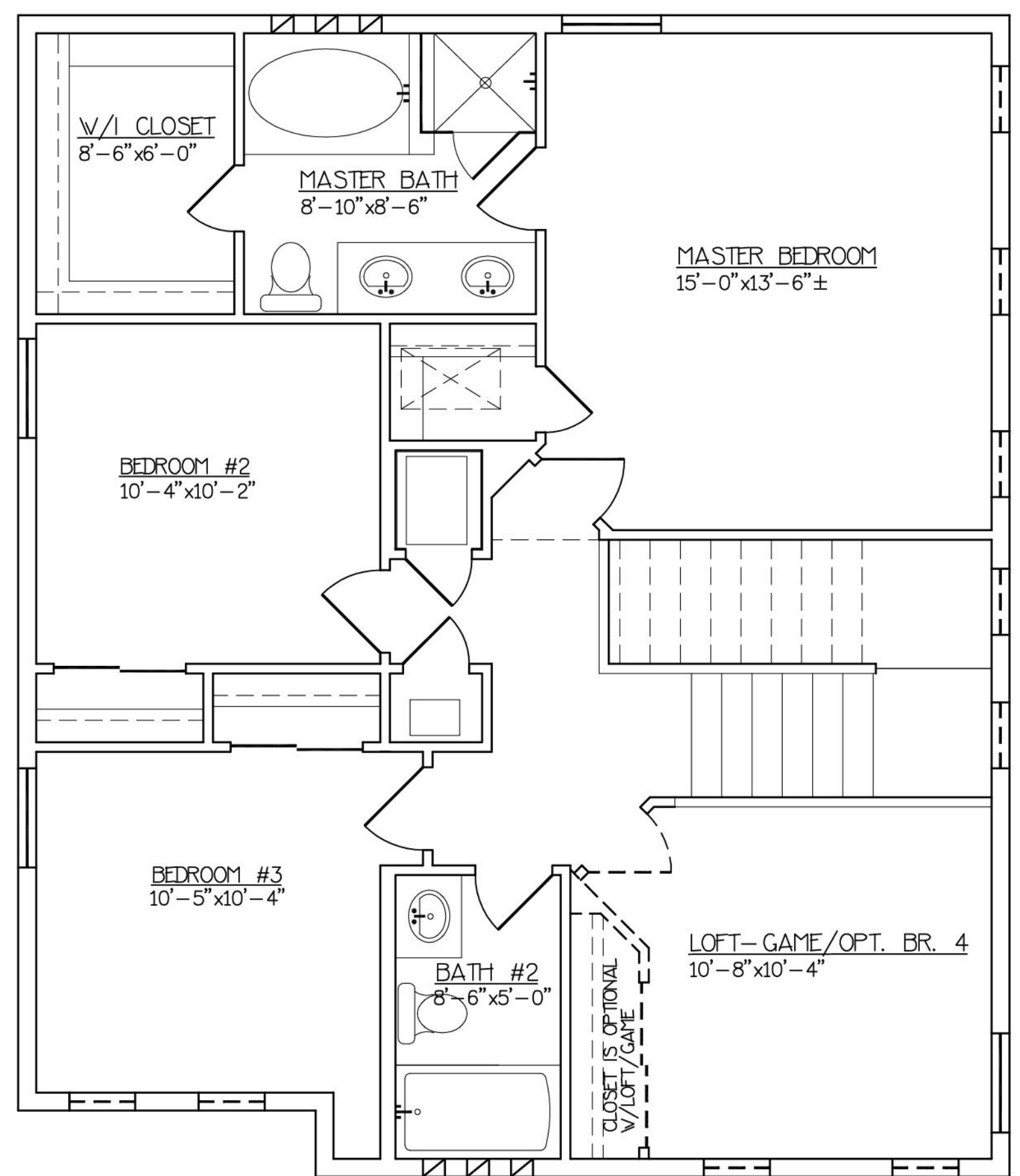
UPSTAIRS FLOORPLAN
