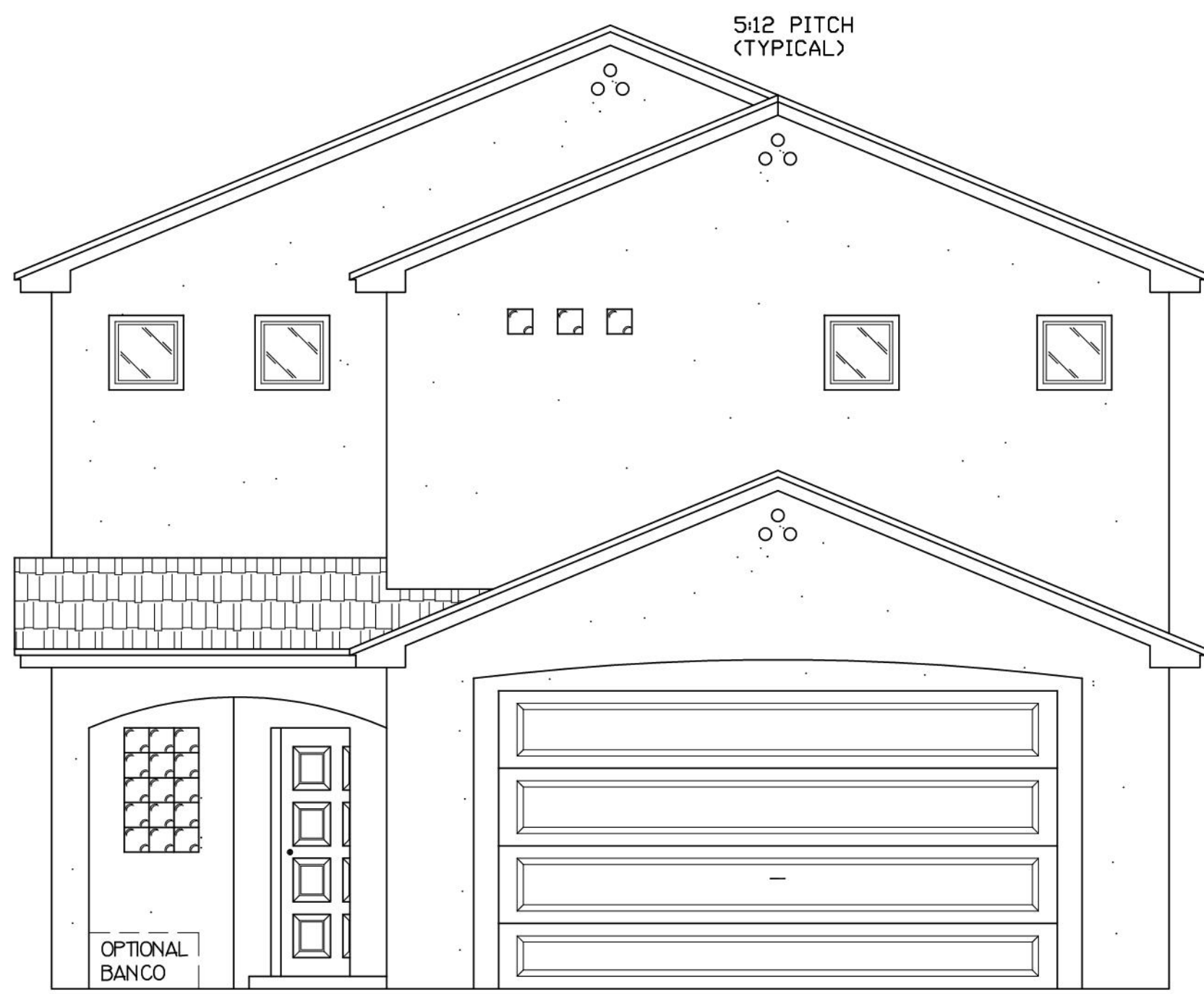
PLAN 1850 FRONT ELEVATION W/GABLE ROOFS
