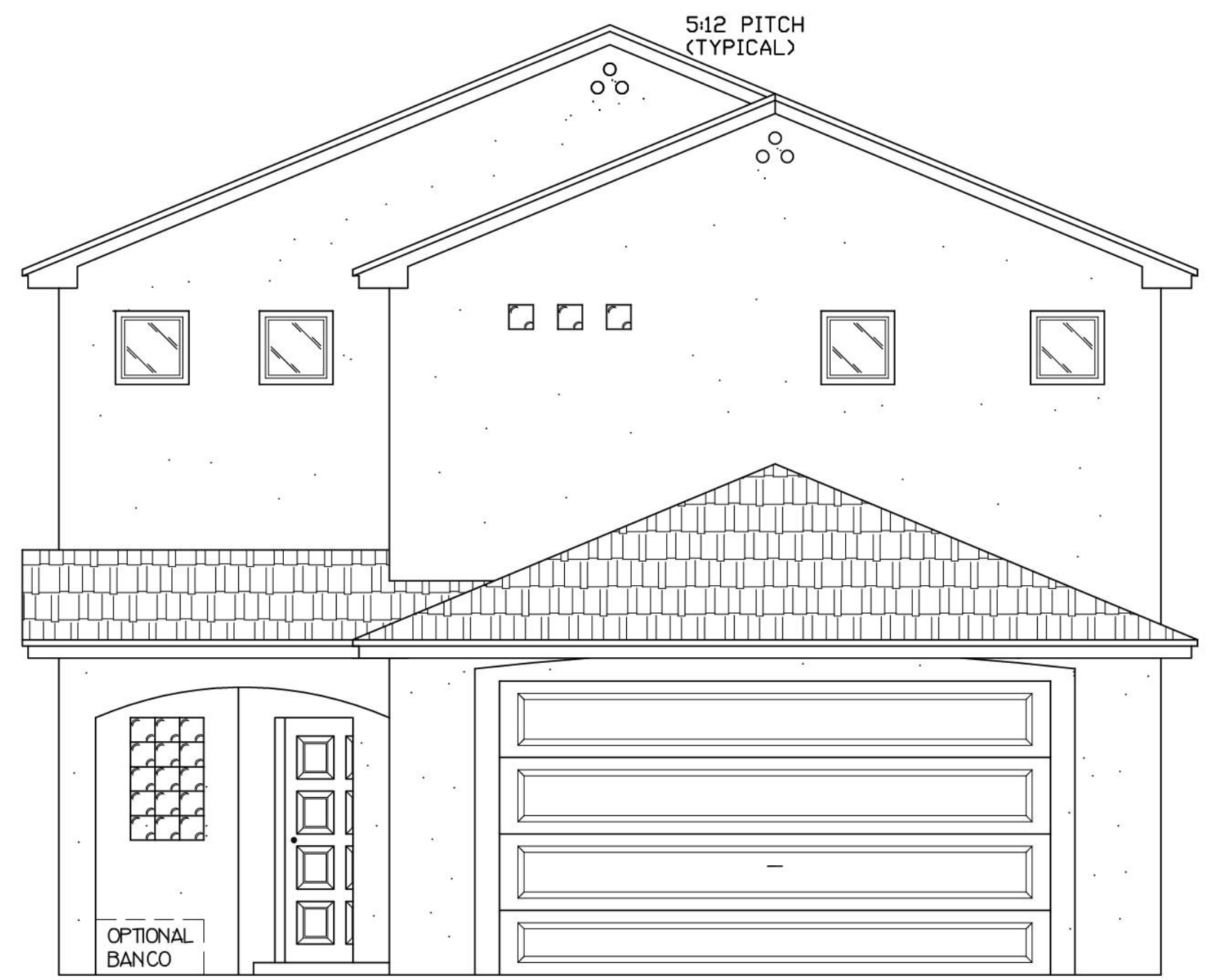
PLAN 1850 FRONT ELEVATION W/HIP ROOF OPTION
