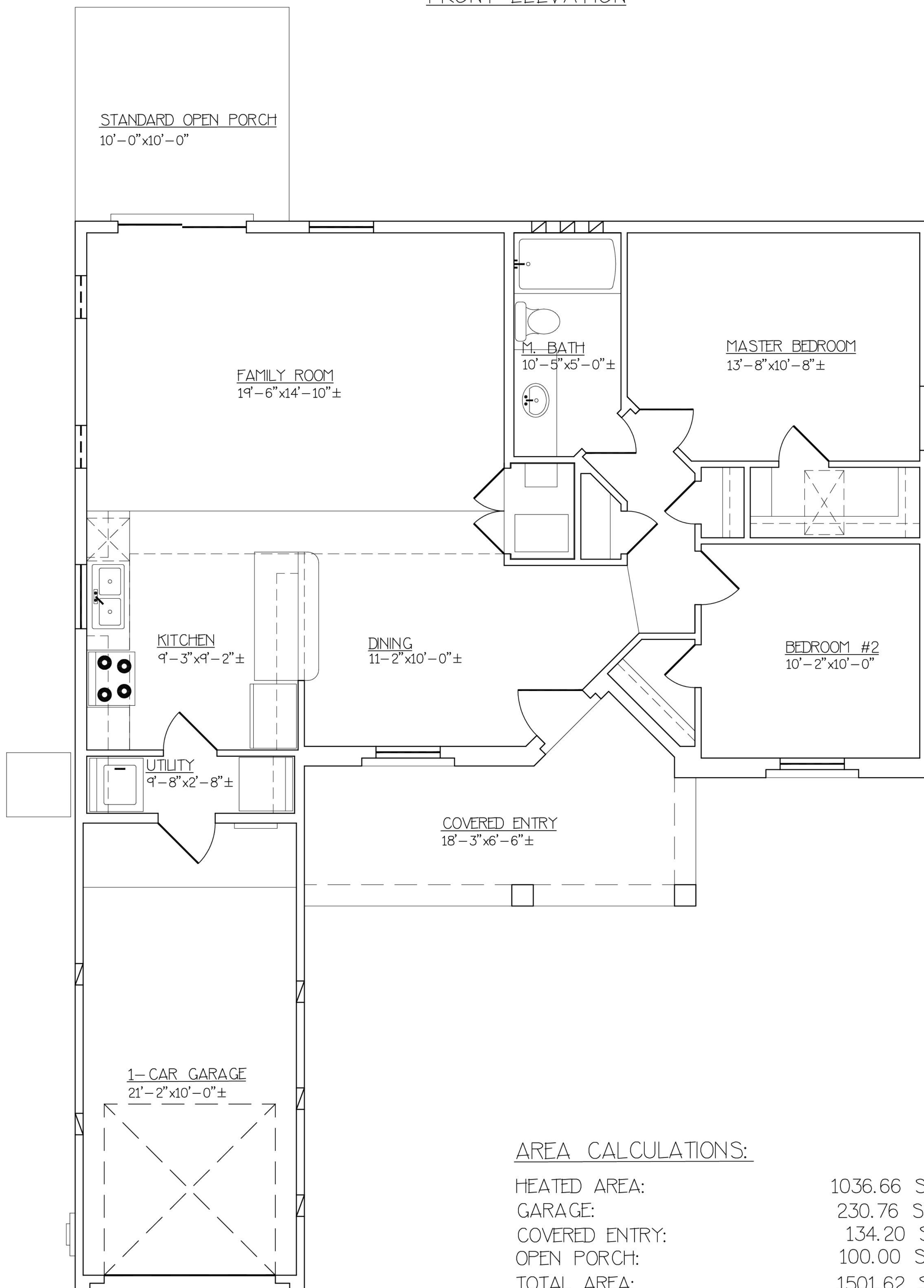
FLOOR PLAN
