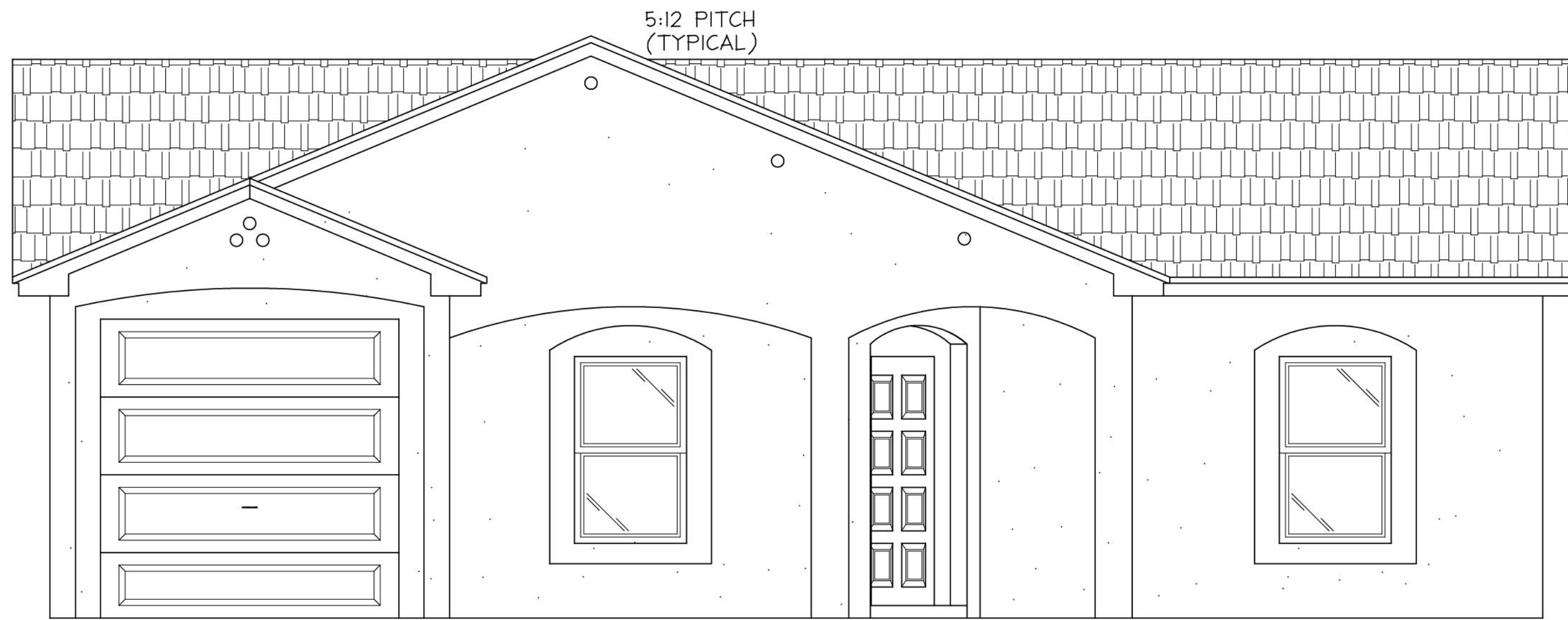
FRONT ELEVATION
